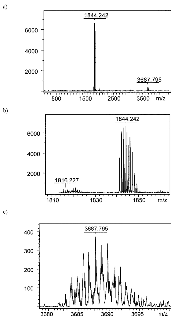
Figure 4. MALDI-TOF spectrum of compound 5 (a) and its zoomed view (b, c), measured without internal standard.
