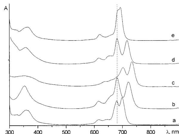
Figure 2. Spectra of 5 in (a) THF + 20% Py; (b) THF over solid NaOH; (c) CHCl 3 /approx. 5 \times 10^{-3} M CF 3 COOH; (d) THF + 20% Py over solid Ni(OAc) 2 ·4H 2 O; (e) THF + 20% Py after addition of a small amount of acetic anhydride.
