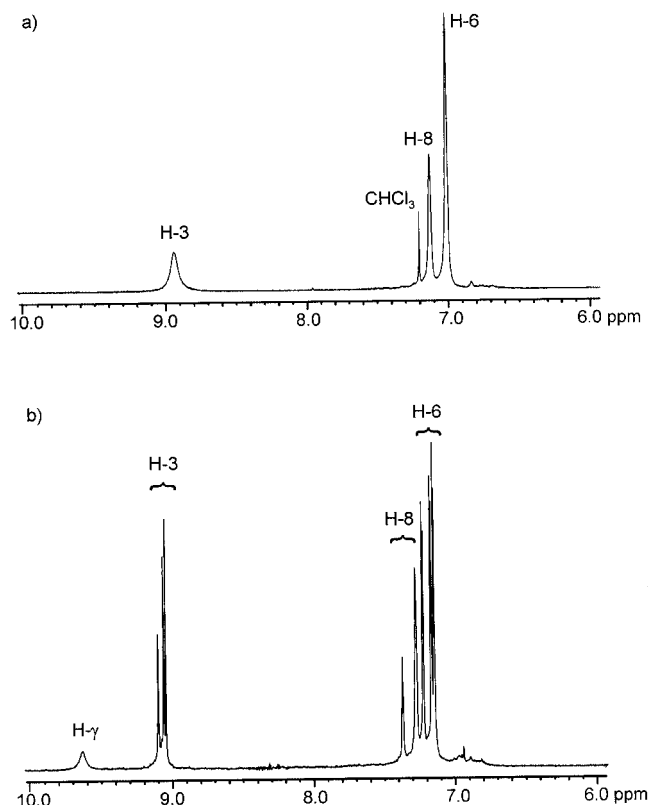
Figure 3. ^1\text{H} NMR (aromatic region) of compounds 4 in \text{CDCl}_3/10\% [\text{D}_8]\text{THF} (a) and 5 in [\text{D}_8]\text{THF} (b).
