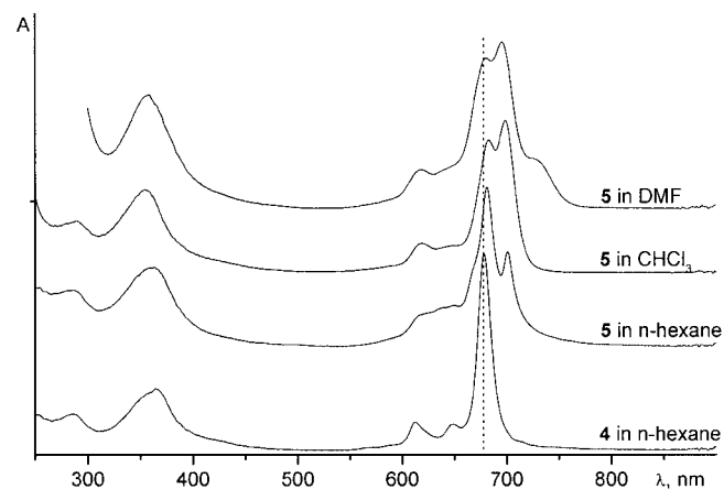
Figure 1. UV/Vis spectra of 4 and 5 in different solvents.
